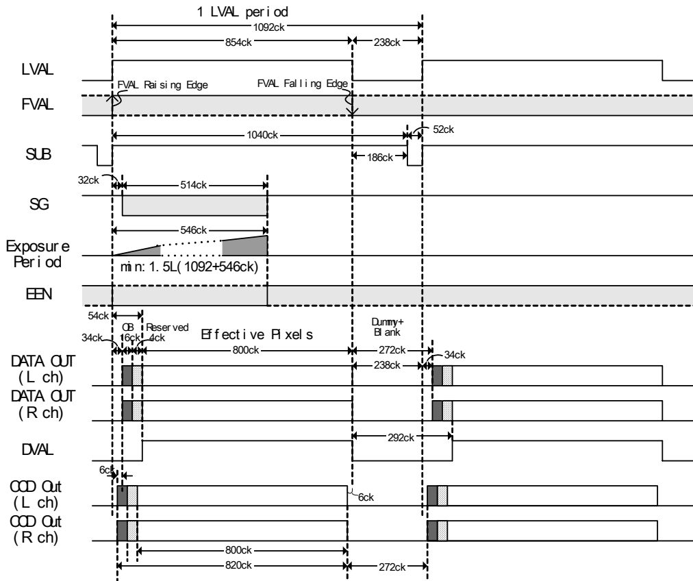
Fig. 19. Horizontal timing dual channel
